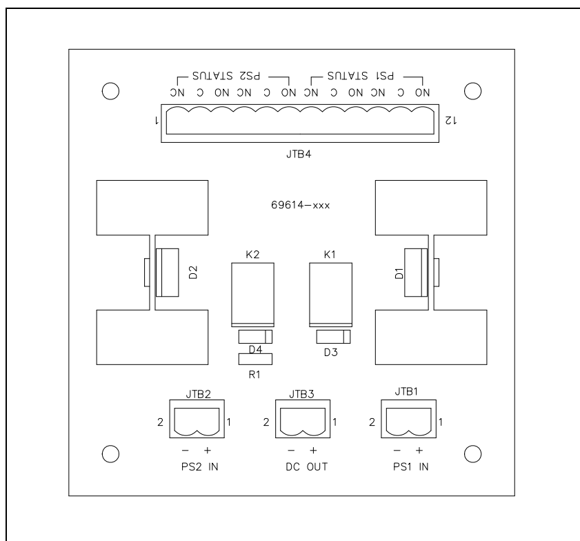
Figure 1. Model 12598-004 Redundant 48 V DC Module
